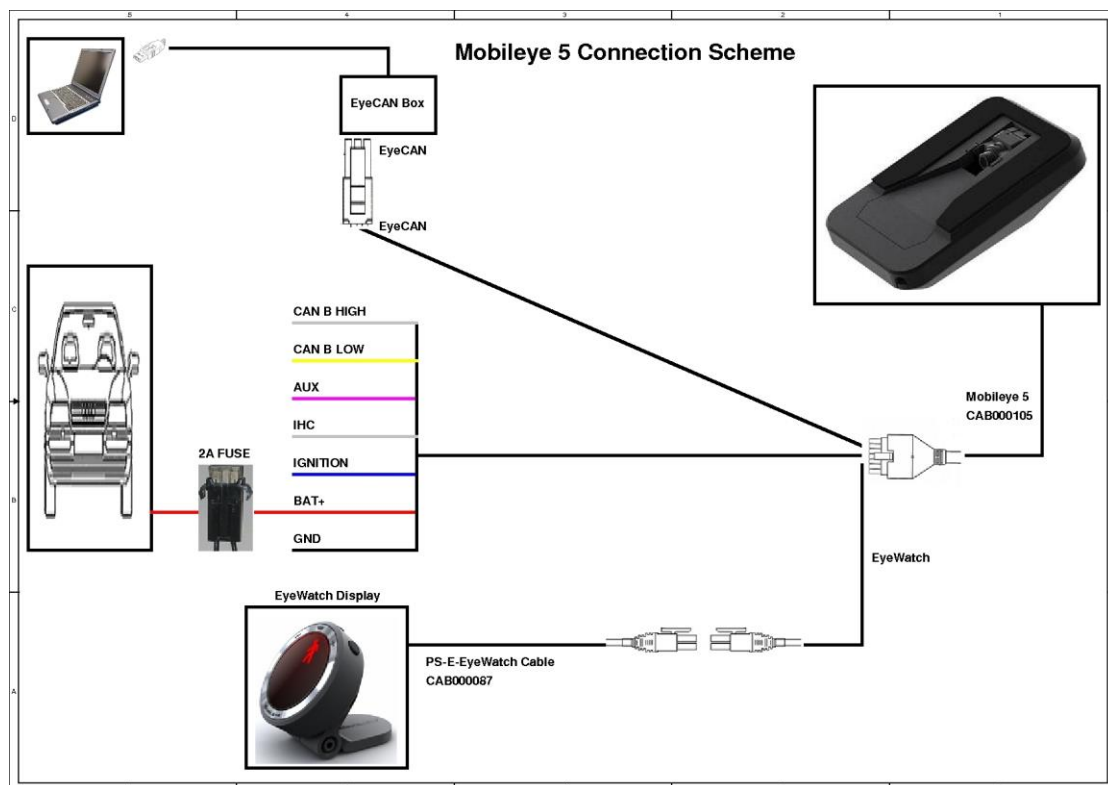
Figure 5: Mobileye 5 connection scheme with EyeCAN
